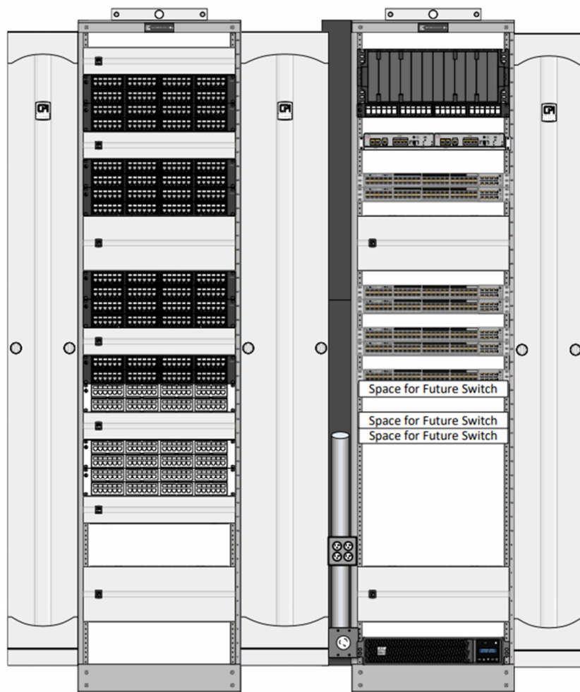
Rack 1 Horizontal
